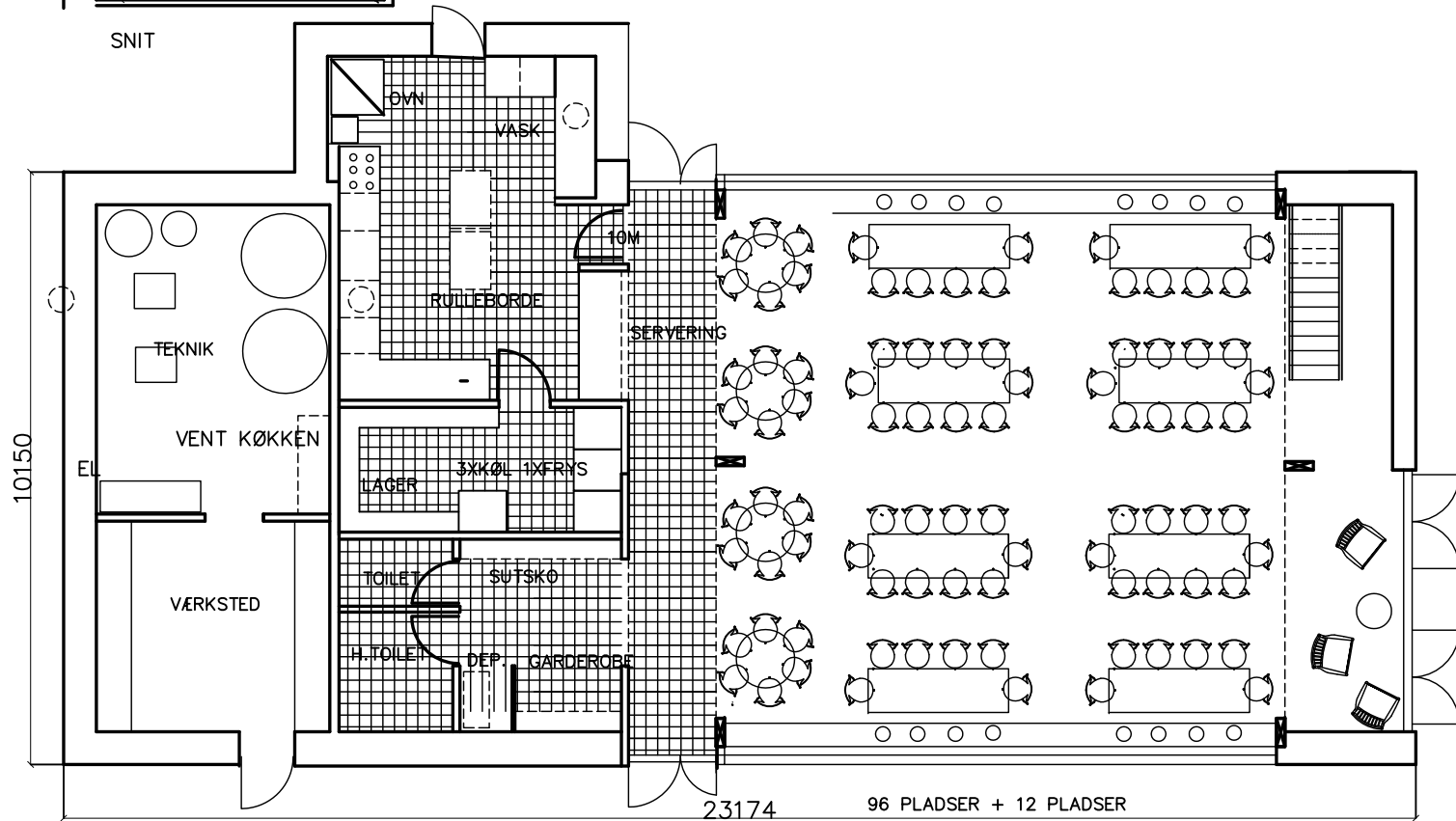
PLAN 10M
